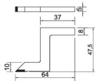
● 3001-4105 For:3001-0105,Range:0-300/0-12"
