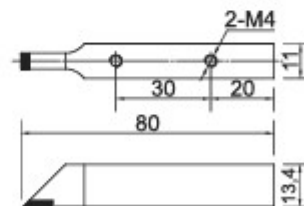
● 3001-4125 For:3001-0125,Range:0-1000/0-40"
