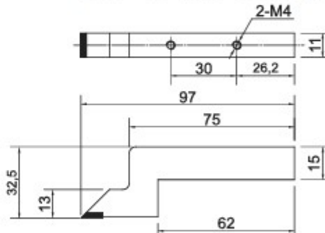
● 3001-4120 For:3001-0120,Range:0-600/0-24"
